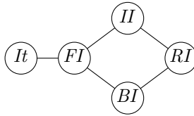
Figure 6.1: Iterator concepts
